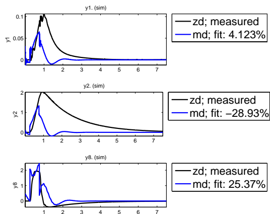
Fig. 3. The fit to validation data for three of the outputs when a full 20th order model is estimated directly.
