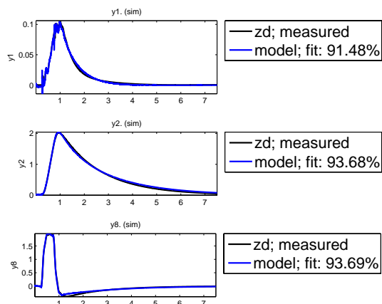
Fig. 4. The fit to validation data for three of the outputs when the “divide-conquer-reunite” strategy is followed.
