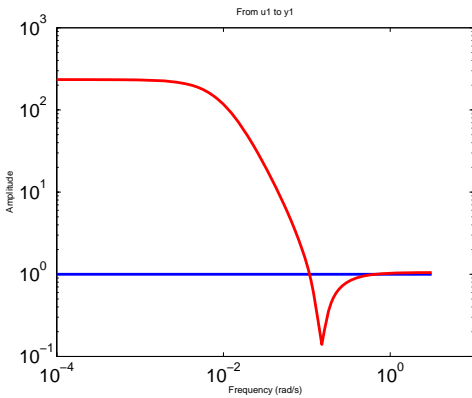
Fig. 5. Amplitude Bode plot of the second order linear equivalent of (23). Straight line: Bode plot of the linear system obtained by ignoring the small nonlinear term.
