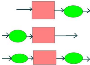
Fig. 6. Typical block oriented models, where squares are linear dynamic systems and ovals are static nonlinearities. Above: A Wiener model. Middle: A Hammerstein model, Below: A Hammerstein-Wiener model.
