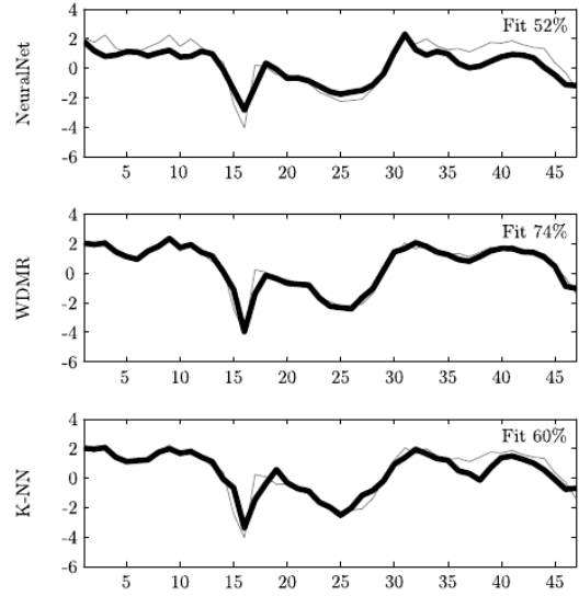
Fig. 2. One step ahead prediction for the models of the Narendra-Li example. Top: Neural Network (18 units); middle: WDMR; bottom: K-Nearest Neighbor (K=15). Thin line: true validation outputs; thick line: model output.
